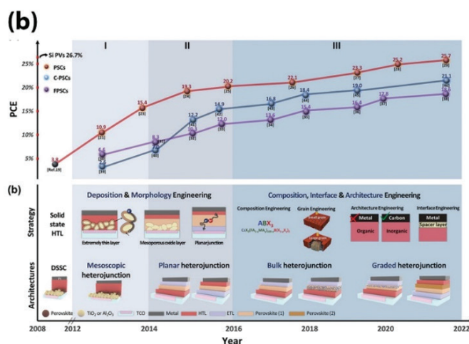
Figure 6 Perovskite semiconductors (a) The evolution of the efficiency of Perovskite Solar Cells (PSCs) from 2008 to 2020 [141]. (b) Chronological evolution of the PCE of Perovskite Solar Cells (PSCs), C-PSCs, and FPSCs and a brief history of schematics for fabrication strategies and device architectures in PSCs (HTL: Hole-Transport Layer, ETL: Electron-Transport Layer, TCO: Transparent Conductive Oxides, PV: Photovoltaic) [142].
