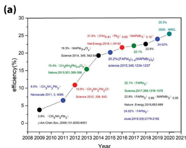
Figure 6 Perovskite semiconductors (a) The evolution of the efficiency of Perovskite Solar Cells (PSCs) from 2008 to 2020 [141]. (b) Chronological evolution of the PCE of Perovskite Solar Cells (PSCs), C-PSCs, and FPSCs and a brief history of schematics for fabrication strategies and device architectures in PSCs (HTL: Hole-Transport Layer, ETL: Electron-Transport Layer, TCO: Transparent Conductive Oxides, PV: Photovoltaic) [142].
