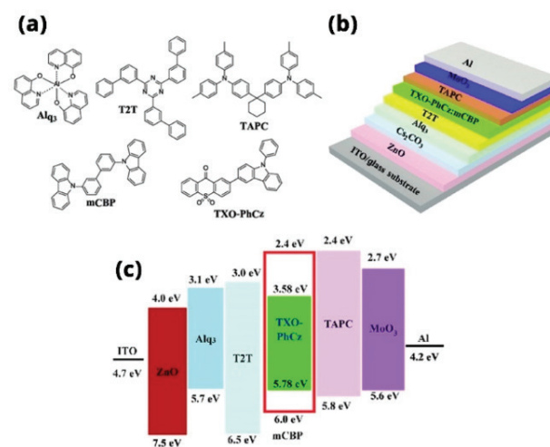
Figure 5) Organic semiconductors. (a) Molecular structures of the organic semiconductors for the inverted OLEDs (b) scheme of the inverted OLEDs and (c) The energy levels of the materials involved in the inverted OLEDs [133].
